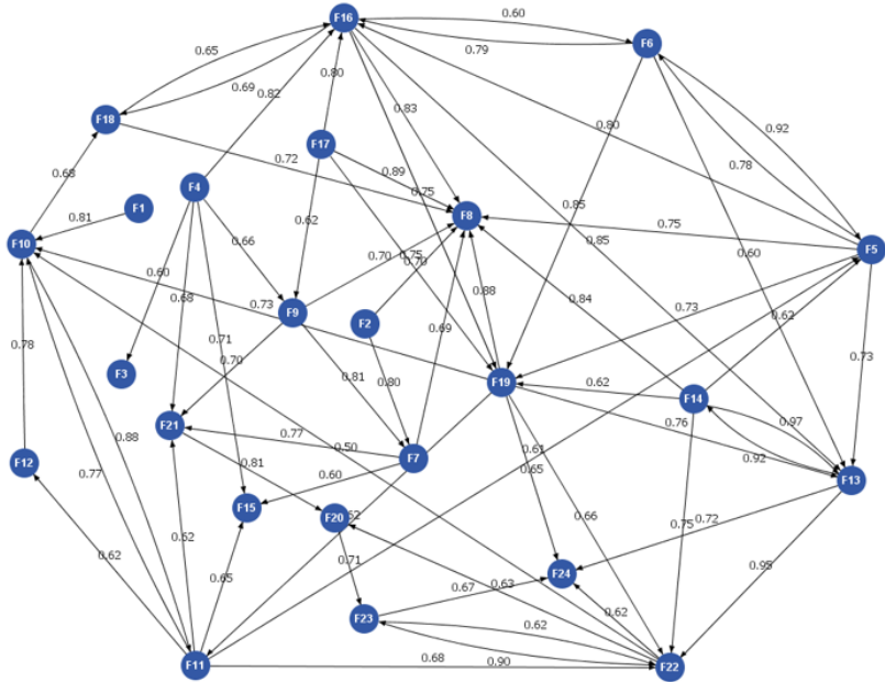
Fig. 3 Graphical structure with important causal relationships
