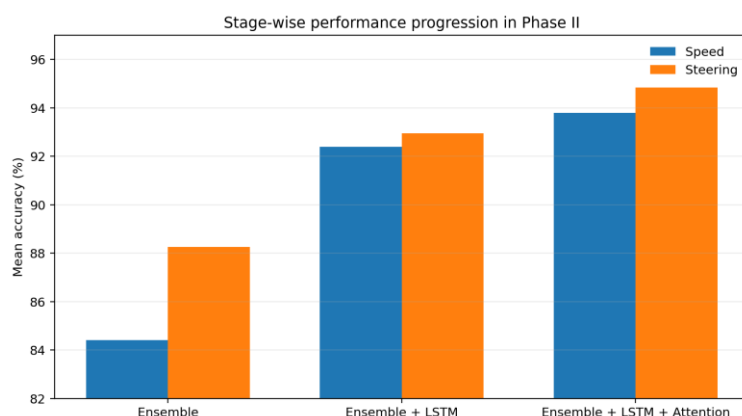
Fig. 8 Mean Phase-II accuracy after stacking only, stacking + LSTM, and stacking + LSTM + attention.
