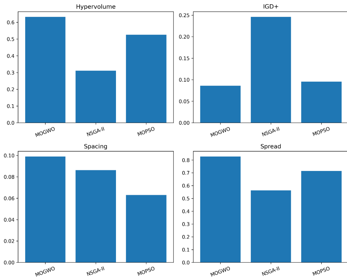
Fig. 4 Comparative results on three meta-heuristics methods based on HV, IGD+, Spacing and Spread measures
